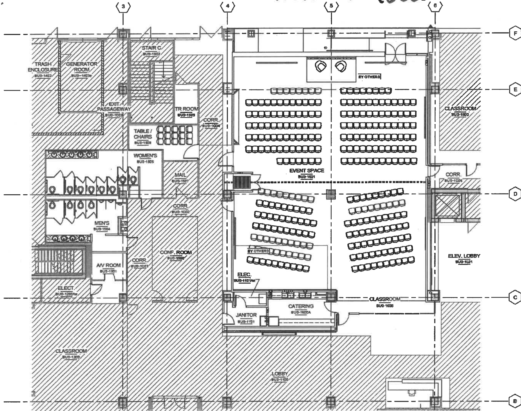
A12 LEVEL 1 FURNITURE PLAN 1/8" = 1'-0"
