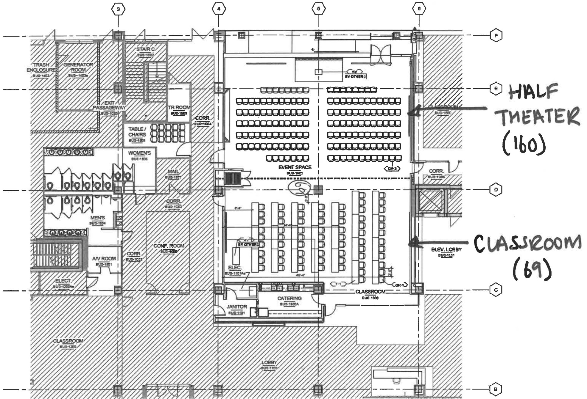
A12 LEVEL 1 FURNITURE PLAN 1/8" = 1'-0"
