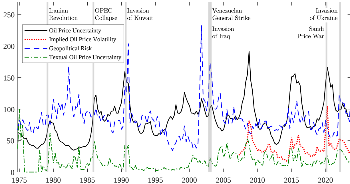
Figure 2: Empirical measures of oil price uncertainty
